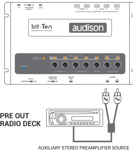
AUXILIARY STEREO PREAMPLIFIER SOURCE
