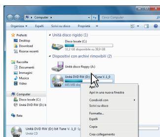
Windows 7
