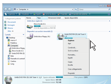
Windows Vista
