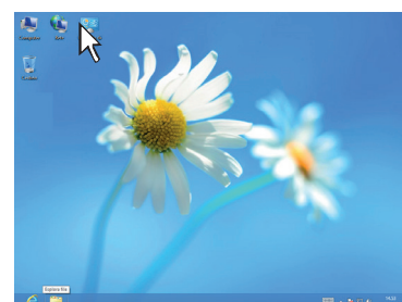
Windows 8 / 10
