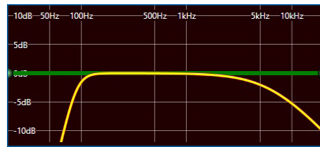
Crossover Frequency 80 Hz @ 24 dB Oct. Hi-pass 2000 Hz @ 6 dB Oct. Low-pass
