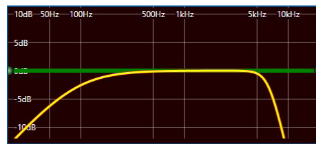
Crossover Frequency 80 Hz @ 6 dB Oct. Hi-pass 2000 Hz @ 24 dB Oct. Low-pass
